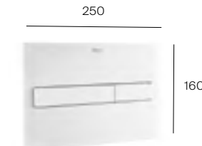
PL7 flush plate Dual flush
